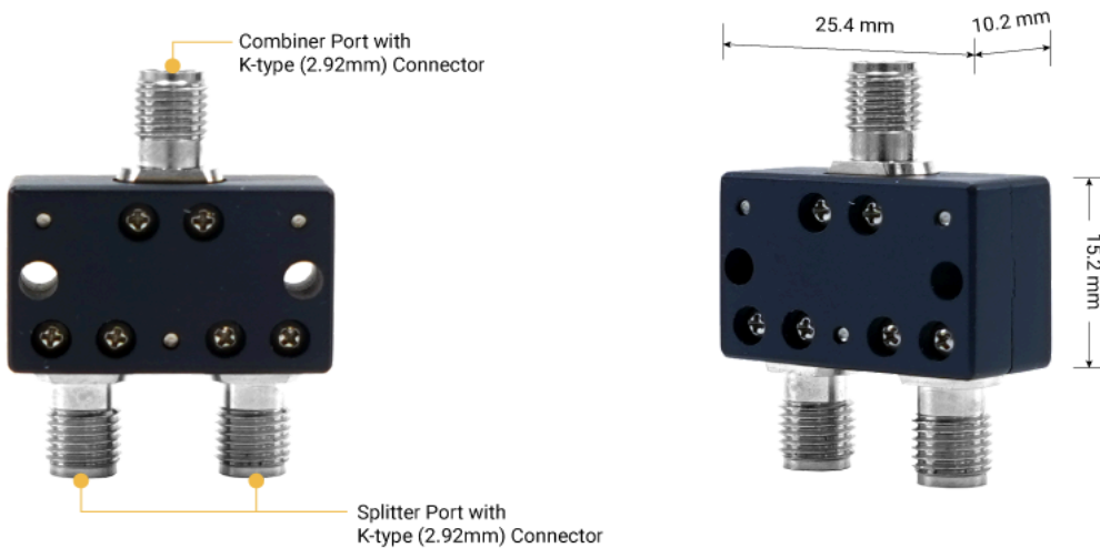
Figure 5. Appearance dimensions & Interface
