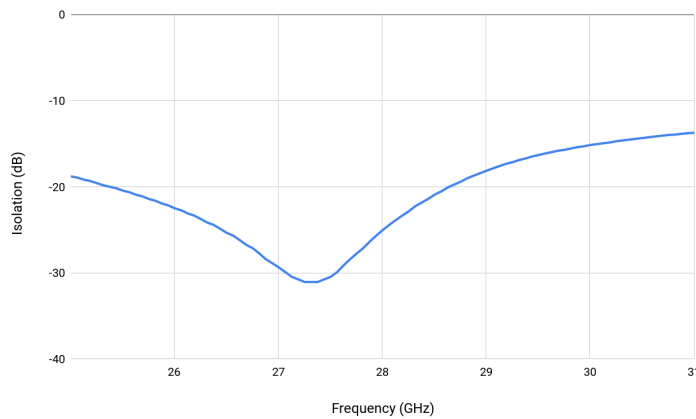
Figure 4. Isolation
