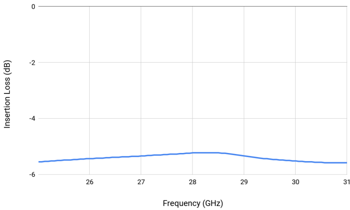
Figure 2. Insertion Loss
