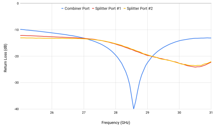
Figure 3. Return Loss
